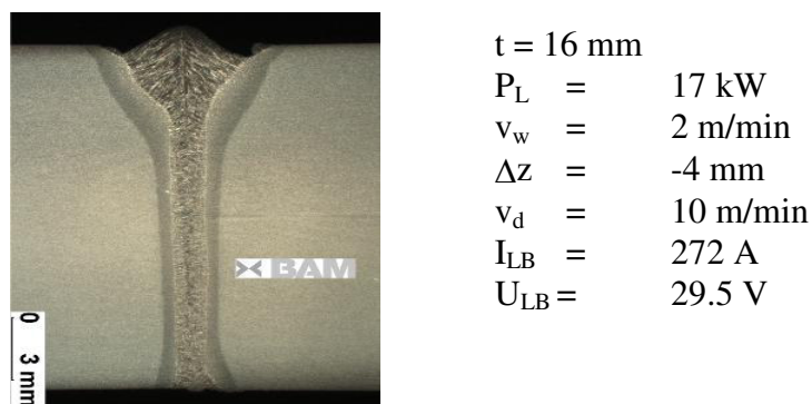
Fig. 5: Positional welding PF (up) 30°
